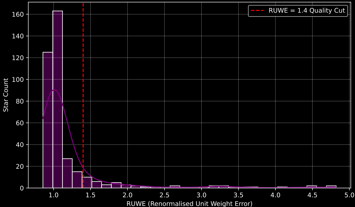
GALAH DR4 Field [6693] RUWE Distribution (n= 376)
