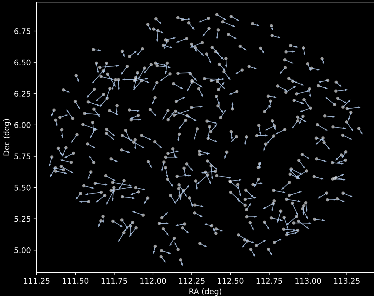
GALAH DR4 Cluster 1 Proper Motion Vectors (n=316)
