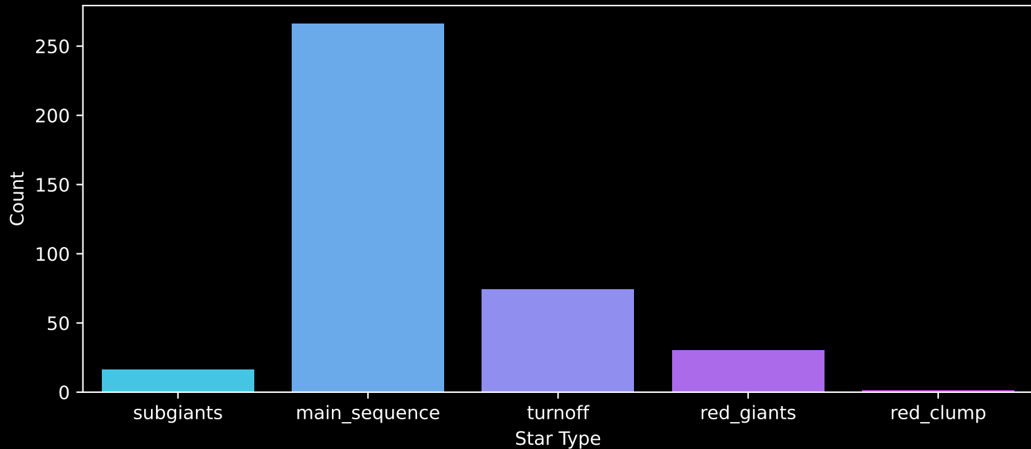
GALAH DR4 Field: [6693] Count plot of Star Type
